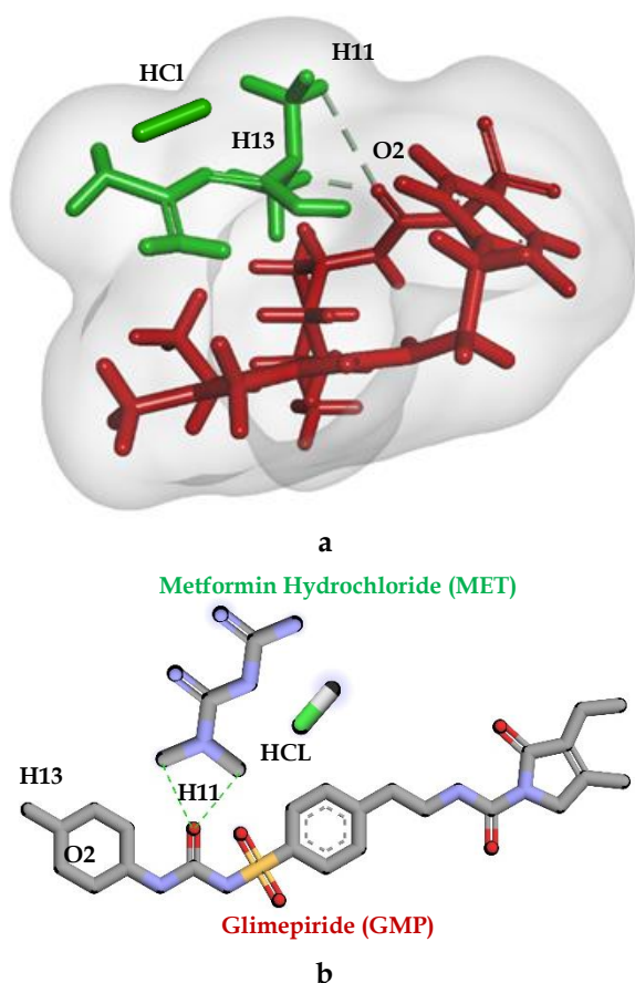
Figure 3. The three-dimensional (a) and two-dimensional (b) interaction of GMP and MET in docking simulations
