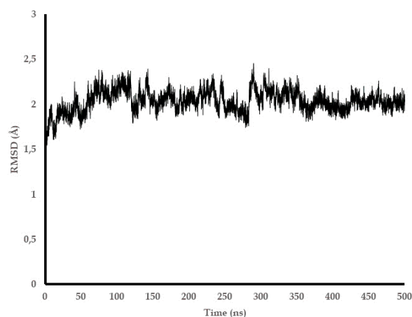
Figure 5. RMSD value during molecular dynamics simulation
