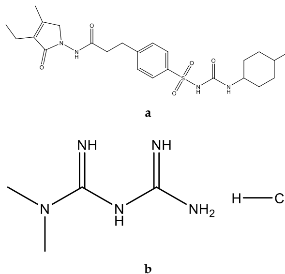
Figure 1. The two-dimensional structure of (a) GMP and (b) MET
