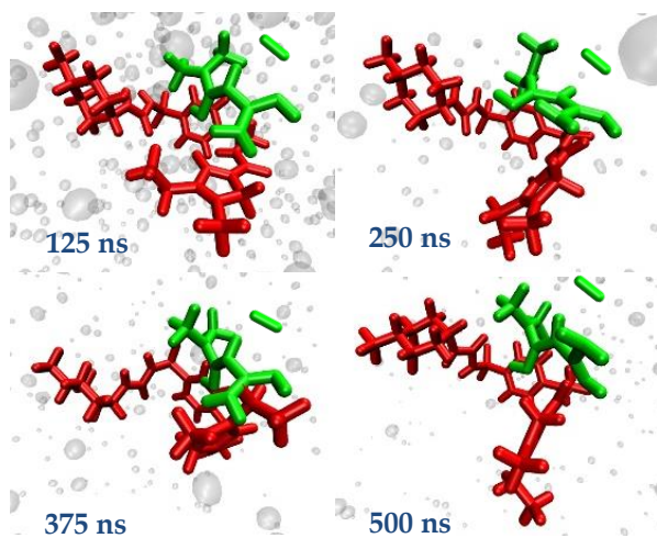
Figure 4. GMP (red) and MET (green) conformation snapshots at 125, 250, 375, and 500 ns
