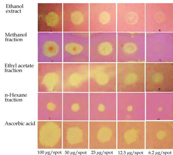
Figure 6. DPPH dot-blot staining of ethanol extract and organic fractions of M. scabra fruit
