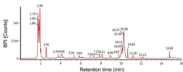
Figure 2. UPLC chromatogram of separated peaks of compounds in the ethanol extract of M. scabra fruits
