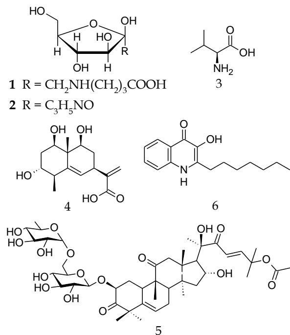
Figure 3. Chemical compounds identified in the ethanol extract of M. scabra fruits
