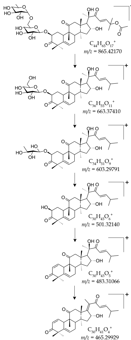
Figure 5. The plausible MS 2 fragmentation of compound 5
