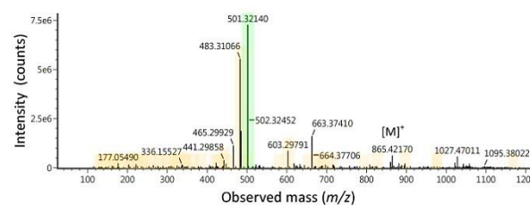
Figure 4. LC-MS/MS spectrum of compound 5
