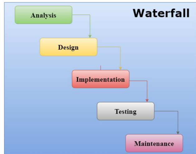
Gambar 1. Metode Waterfall
